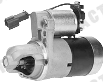
SM-1611 1.2kw,CW,8T,PMGR
