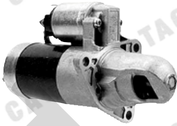
SM-1546 1.7kw,CCW,12T,PMGR
