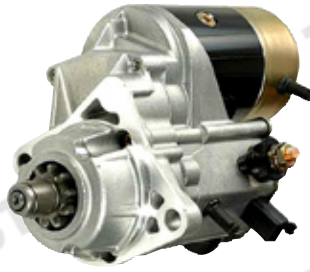
SN-8501 2.5kw,CW,10T
