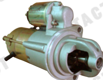
SD-1692 1.7kw,CW,9T,PG260M
