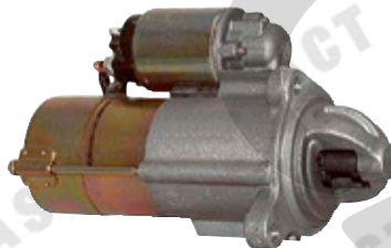
SD-1912 1.7kw,CW,9T,PG260M
