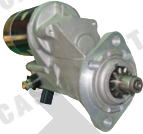
SN-8416 2.5kw,CW,11T
