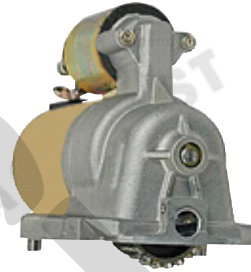
SF-2198 1.5kw,CCW,22T,PMGR
