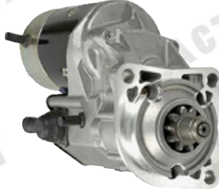
SN-8506 2.5kw,CW,10T
