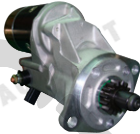
SN-25158 2.5kw,CW,15T
