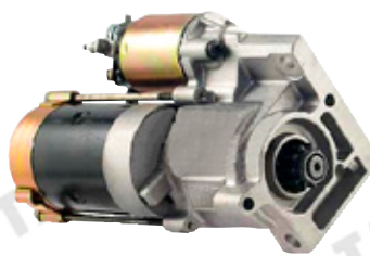
SM-1408 1.2kw,CW,10T,OSGR
