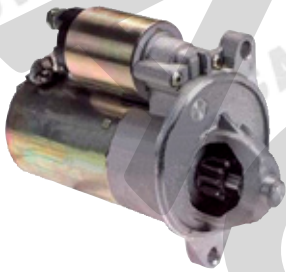
SF-1956 1.5kw,CW,10T,PMGR
