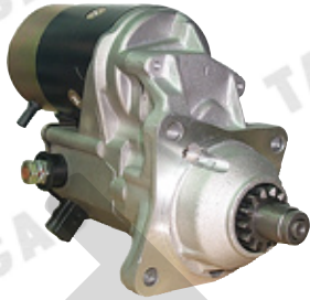
SN-2416 2.7kw,CW,13T
