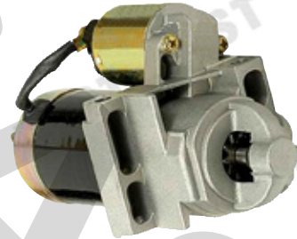
SD-1999 1.4kw,CW,11T,PG260G
