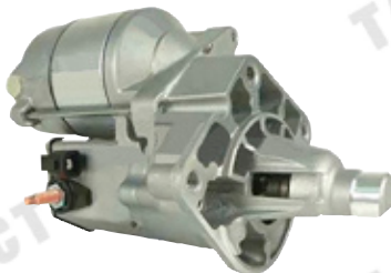
SN-2670 1.2kw,CW,10T
