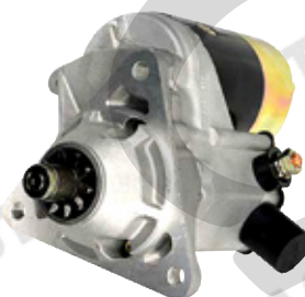
SN-8097 2.5kw,CW,10T
