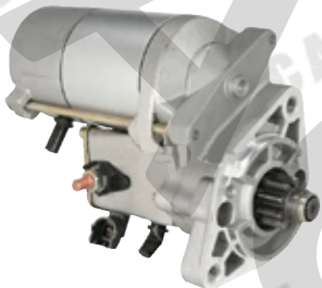
SN-2662 2.0kw,CW,10T
