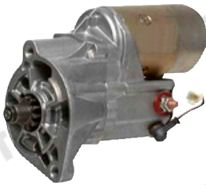
SN-1730 4.5kw,CW,11T
