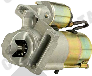
SD-1688 1.7kw,CW,11T,PG260M
