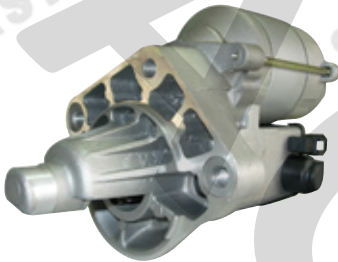
SN-1527 1.2kw,CW,10T
