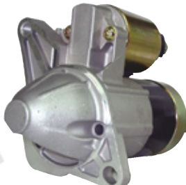
SM-1992 1.2kw,CW,8T,PMGR
