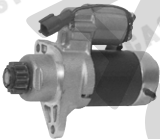
SH-1441 1.7kw,CCW,13T,PMGR
