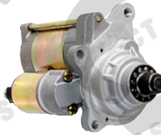
SF-2215 3.0kw,CW,12T,OSGR
